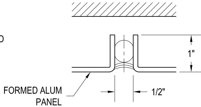
2 TYPICAL DETAIL
