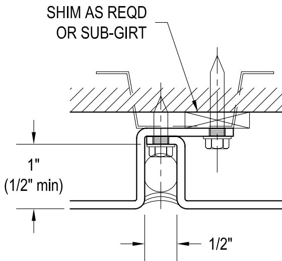
4 TYPICAL DETAIL
